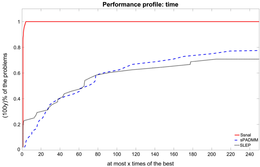
Fig. 1 Performance profiles of SSNAL, sPADMM, and SLEP on UCI data sets with randomly generated groups
