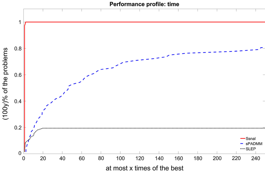
Fig. 2 Performance profiles of SSNAL, sPADMM, and SLEP on UCI data sets with simulated groups
