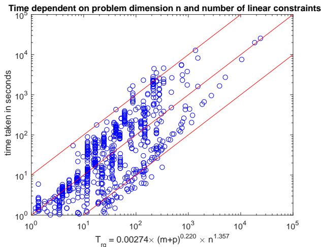
Figure 1: Time T taken to solve 707 SDP instances versus the times estimated based on regression T_{\text{rg}} = 0.00274 (m + p)^{0.220} n^{1.357} .
